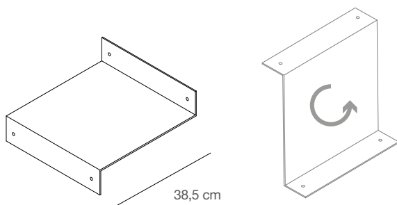
MENSOLA IN METALLO (REVERSIBILE) METAL SHELF (REVERSIBLE)
